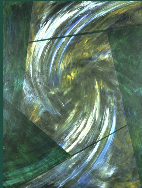
Ace Of Earth Good fortune, success in the world's pursuits. "View From Hubble" 48in. x 36in.
